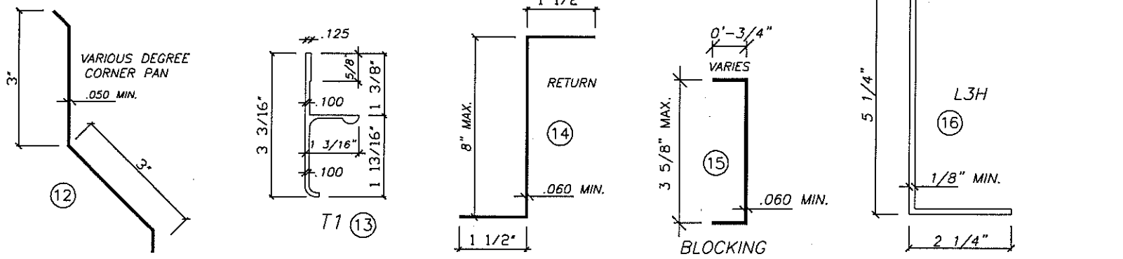
VARIOUS TYPES OF F-TRACK NOT SHOWN
