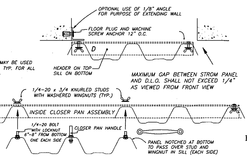
PLAN VIEWS DETAIL 12 A, B, C & D
