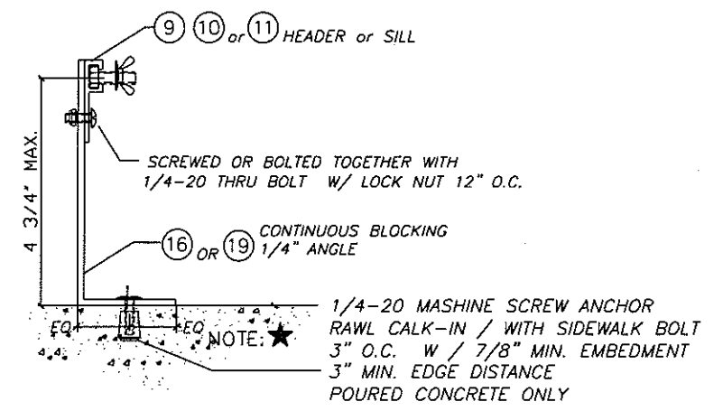
DETAIL 21 ADJUSTABLE HEADER OR SILL
