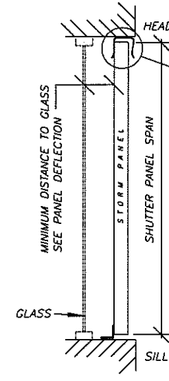
DETAIL 4 ON SHEET 2
