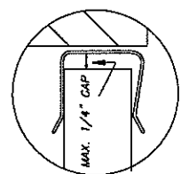
MAXIMUM GAP BETWEEN PANEL AND HEADER IS 1/4" (TYP.)
