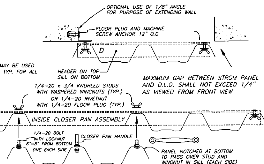
PLAN VIEWS DETAIL 12 A, B, C & D
