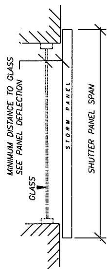
DETAIL 13 ON SHEET 3
