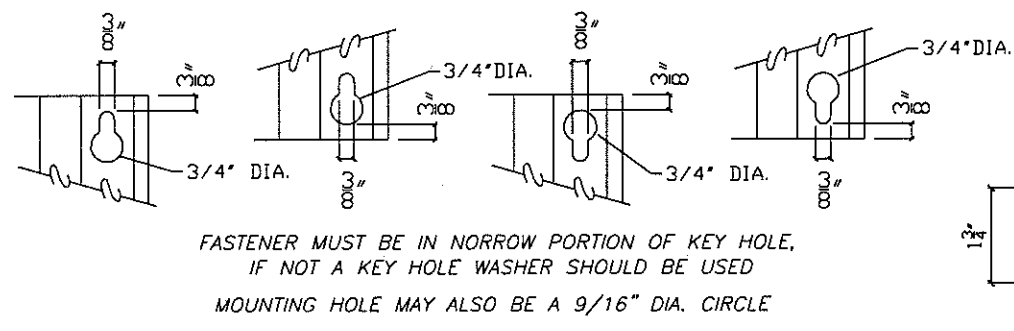
KEY HOLE WASHER
